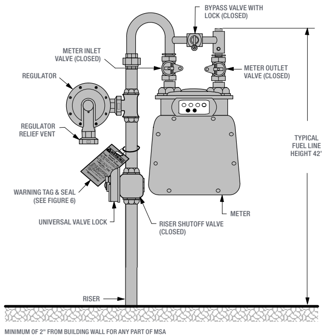
Typical A425 through A1000 gas meter set assembly
