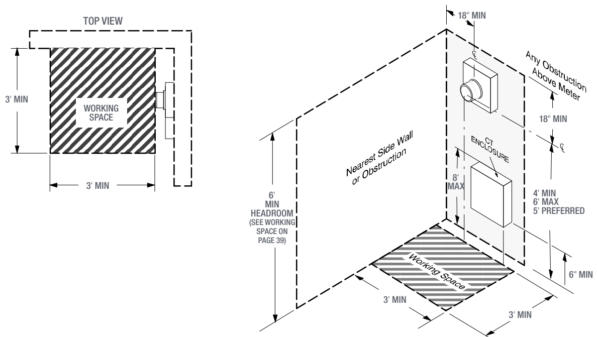
Figure 19 Meter base/socket minimum clearances, without switchgear
