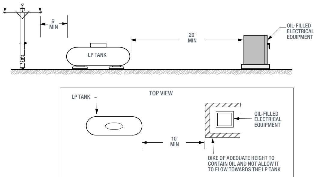
Figure 11 Minimum clearances from oil-filled equipment to LP, hazardous liquid, or fuel tanks
