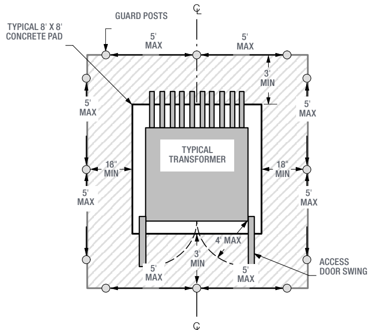
Figure 14 Guard post location requirements
