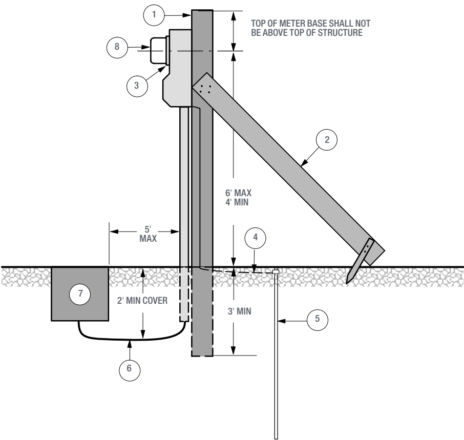
Figure 37 Temporary underground service installation
