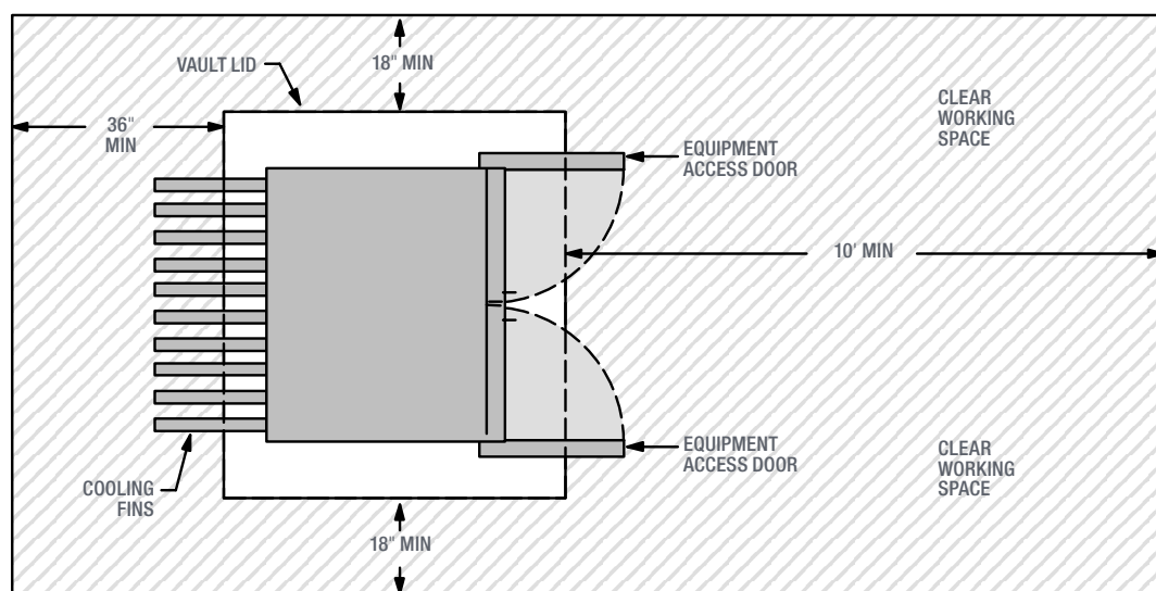
Figure 13 Plan view of padmount equipment clear working space
