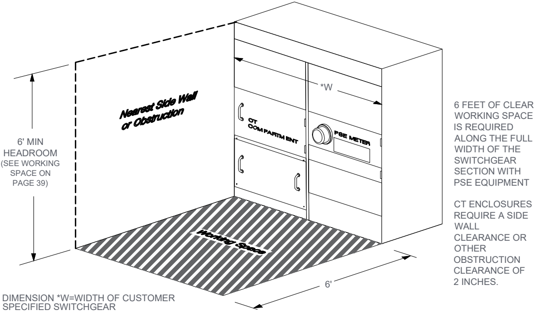
Figure 20 Switchgear installed meter and current transformer minimum clearances
