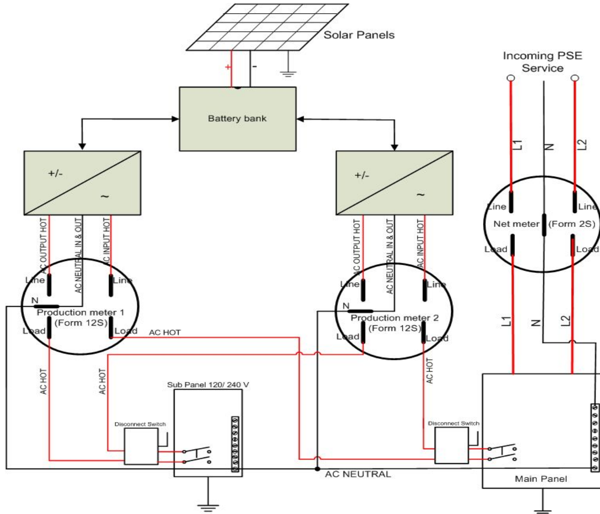
PV System with Battery Backup – Twin 12S Meter Configuration
