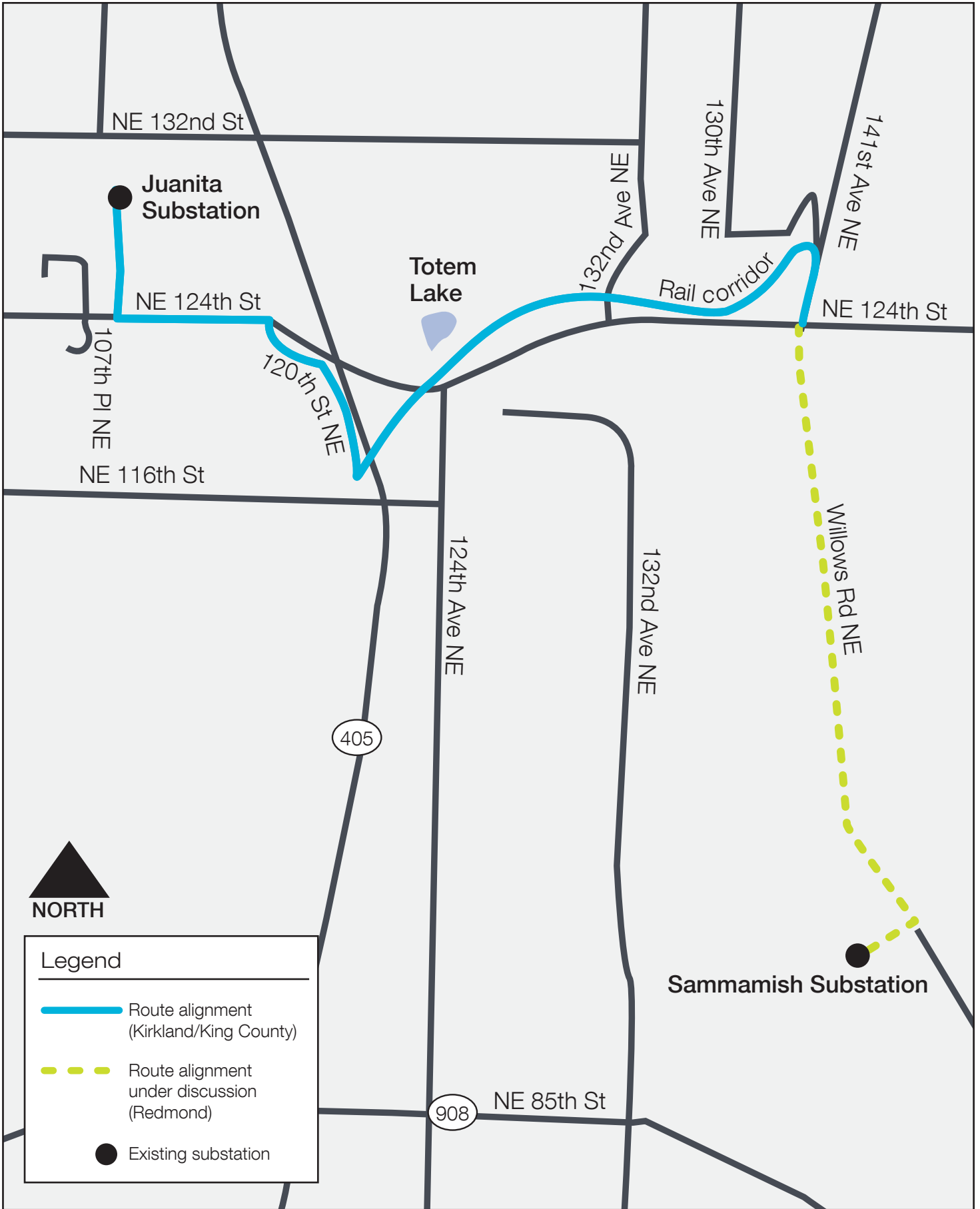
Kirkland/Redmond electric system improvements Sammamish-Juanita 115 kV transmission line
