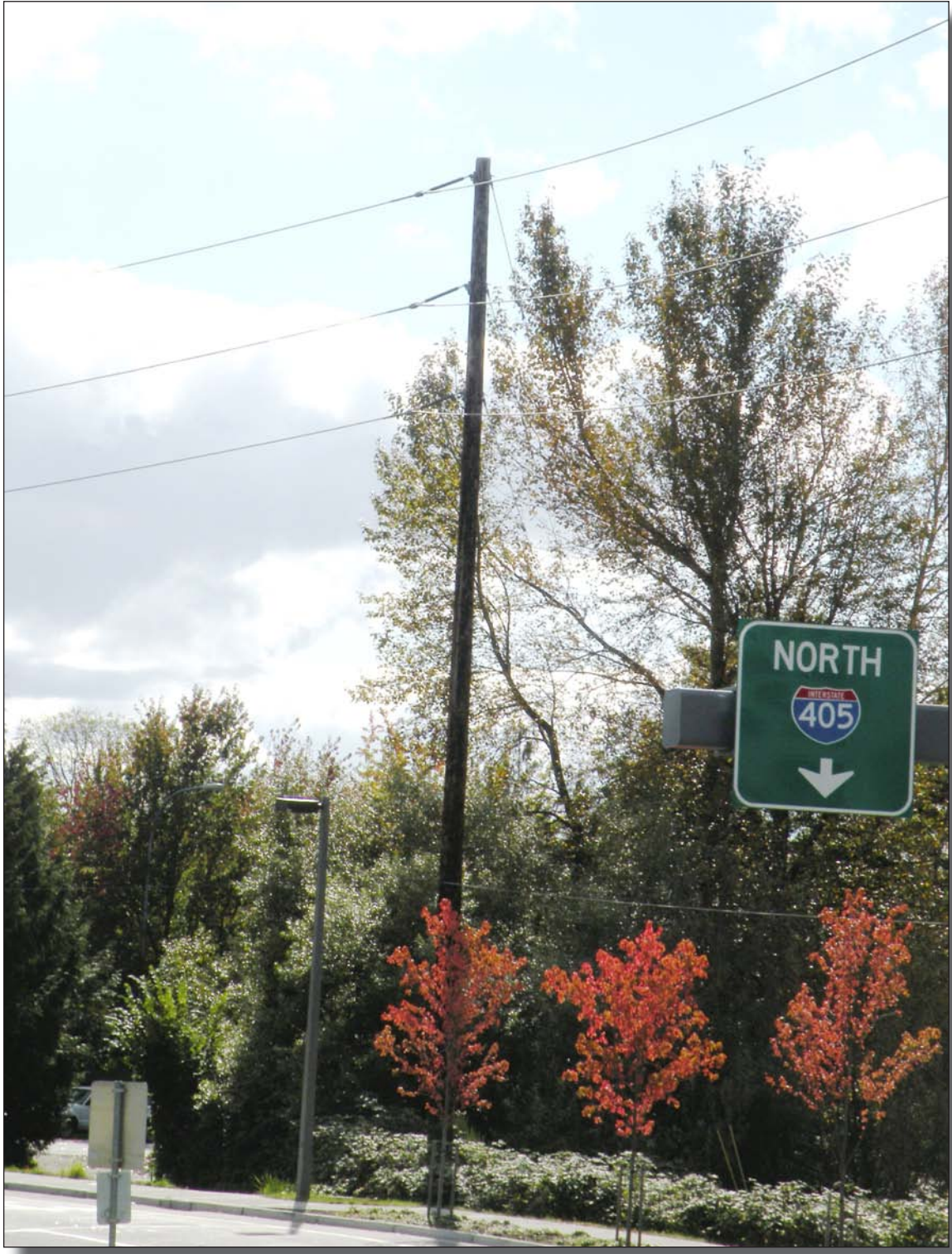
Single-circuit 115 kV wood pole without distribution underbuild
